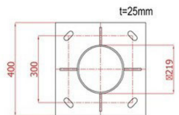
BASE PLATE
