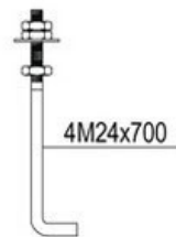
ANCHOR BOLT
