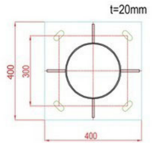
BASE PLATE
