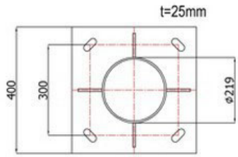
BASE PLATE
